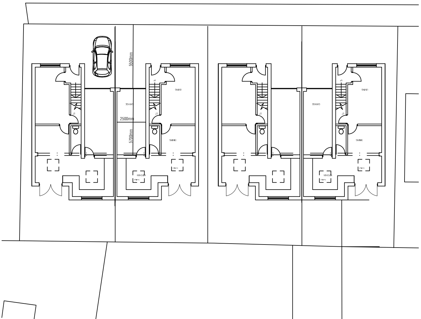
Proposed Site Plan (Scale 1:200 @ A4)
